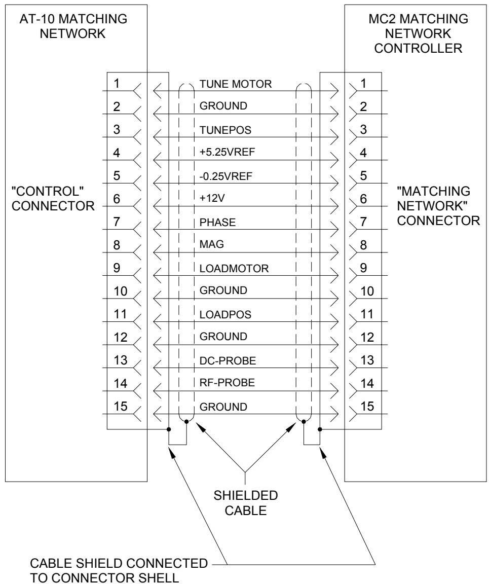
EJAT10 Control Interface Connections
