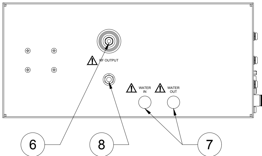
EJAT10 Rear Panel, With Stud Terminal Output
