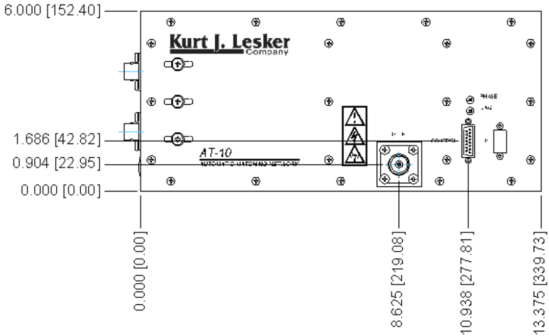
EJAT10 Side View
