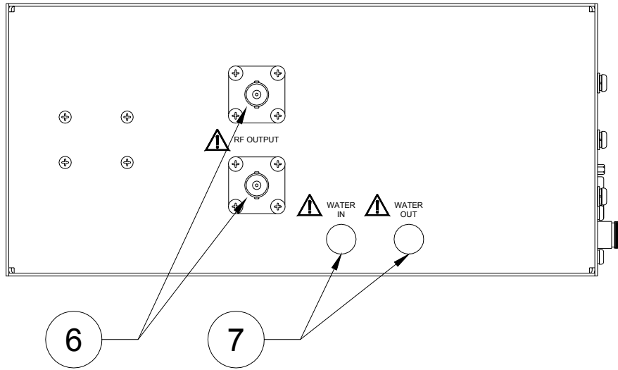
EJAT10 Rear Panel, With Dual “C” Output Connectors
